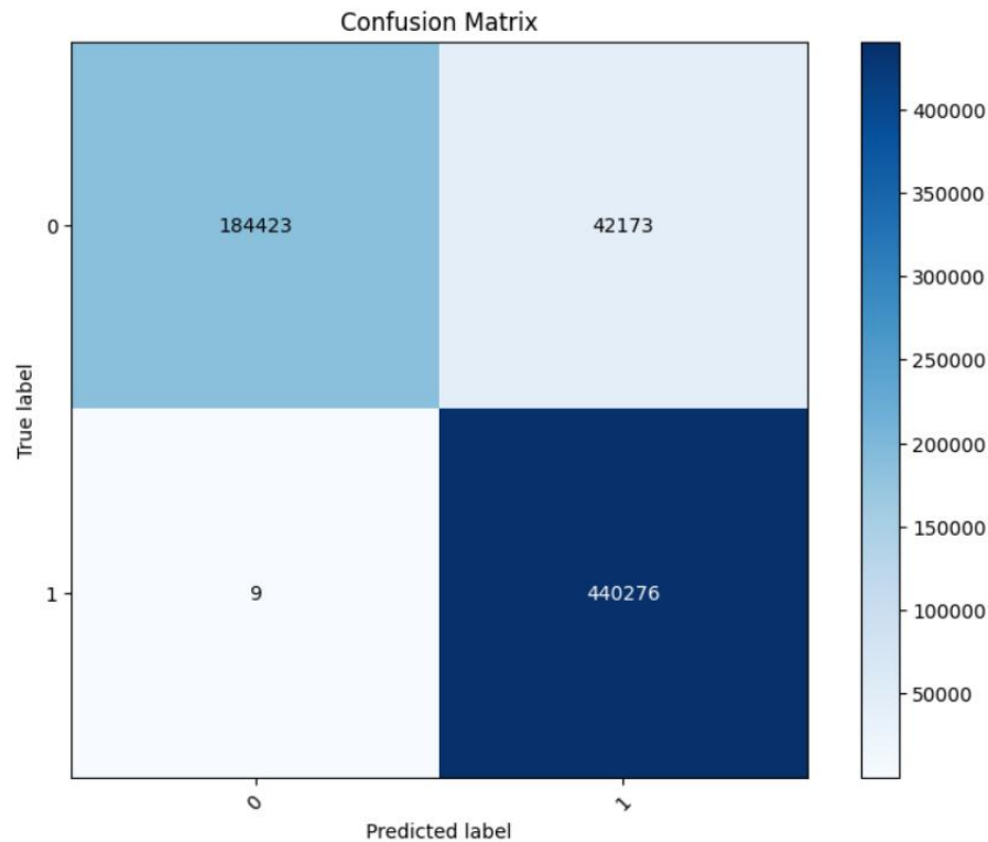
Figure 14 Confusion Matrix
